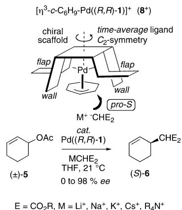
Figure 2. Wall-and-flap cartoon model 20 for asymmetric alkylation involving Pd complexes of (R,R)\text{-1} , with the asymmetric alkylation of cyclohexenyl acetate ( 5 ) as an example.
