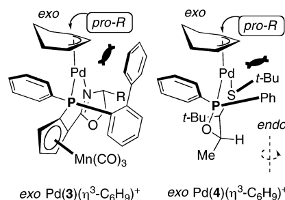
Figure 1. Pd( \eta^3 - c -C 6 H 9 ) complexes of the P,X-ligands 3 12 and 4 13 designed for asymmetric alkylation of cycloalkenyl esters, illustrating the two control elements: exo/endo biasing and activation trans to P.
