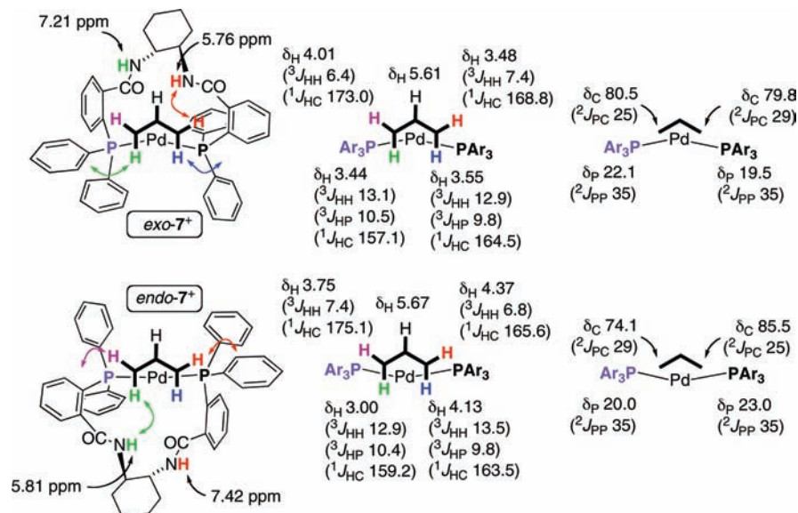
Figure 4. Color-coding showing the static P,P–Pd- \eta^3 -allyl unit during interconversion ( k = 2.6(\pm 0.3) \text{ s}^{-1} , \text{CD}_2\text{Cl}_2 , 25^\circ\text{C} ) of monomeric exo-7 + and endo-7 + with selected NMR data ( \delta/\text{ppm} , J/\text{Hz} ) and NOE contacts.
